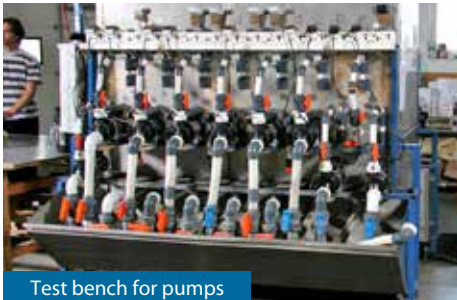
Test bench for pumps
